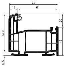
5505 Export
