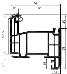
5504 Export
