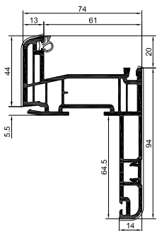
5515 Export
